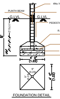
FOUNDATION DETAIL
