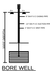
BORE WELL
