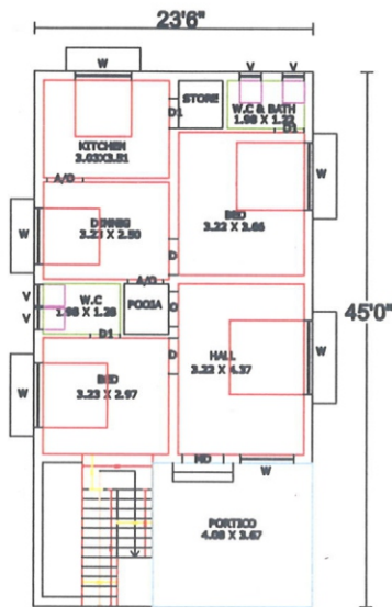
EXIST.GROUND FLOOR PLAN
