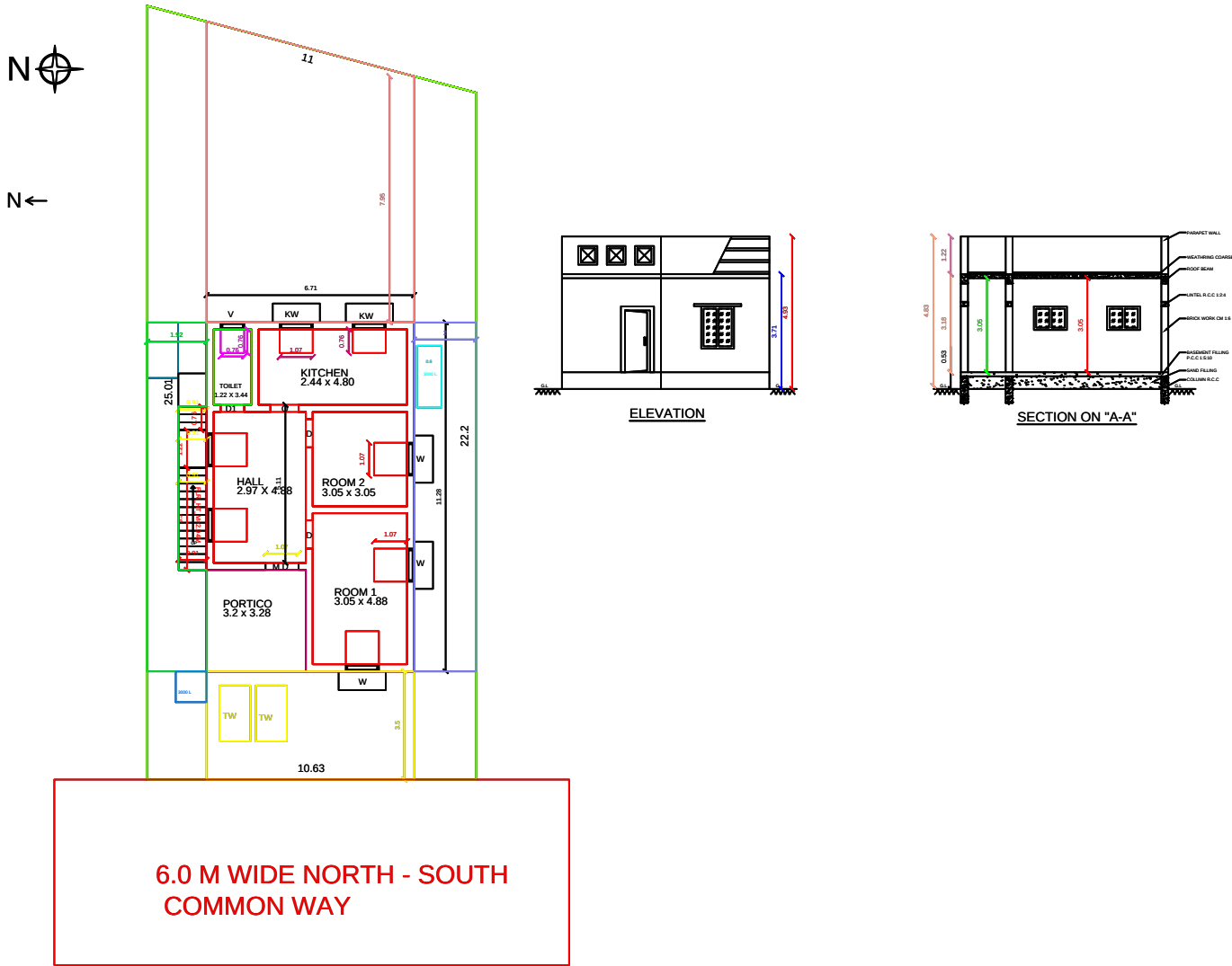
SITE PLAN CUM PROPOSED GROUND FLOOR PLAN
