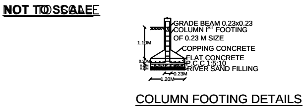
COLUMN FOOTING DETAILS
