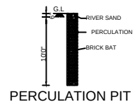
PERCULATION PIT
