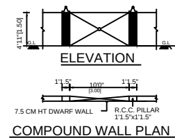
COMPOUND WALL PLAN
