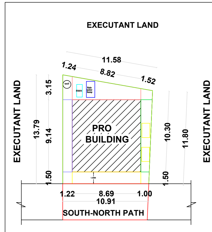
SITE PLAN & KEY PLAN (1:100)
