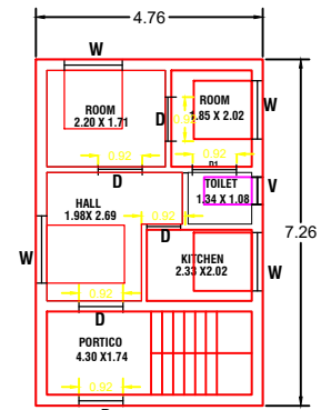
PRO., GROUND FLOOR PLAN
