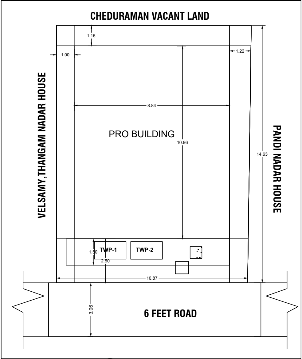
SITE PLAN
