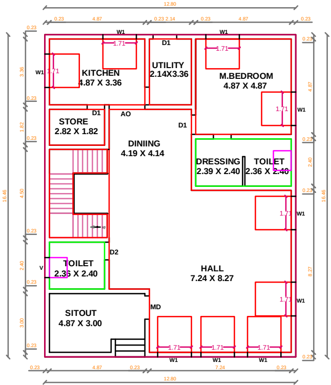
GROUND_FLOOR_PLAN GROUND FLOOR PLAN PROPOSED
