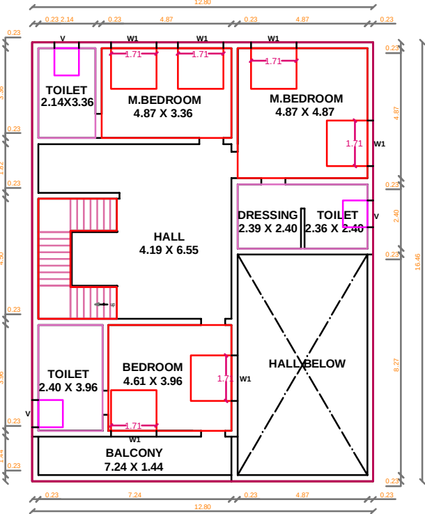
FIRST_FLOOR_PLAN FIRST FLOOR PLAN PROPOSED
