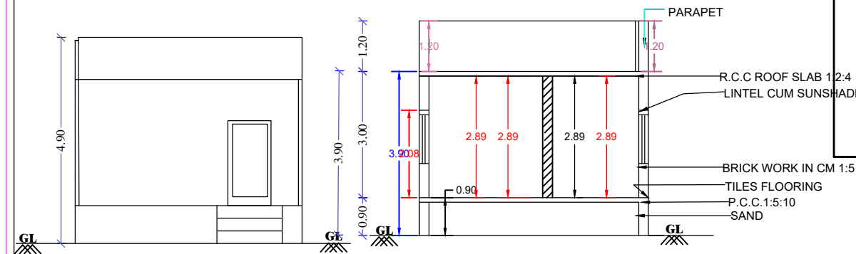
SECTION ON A-E
