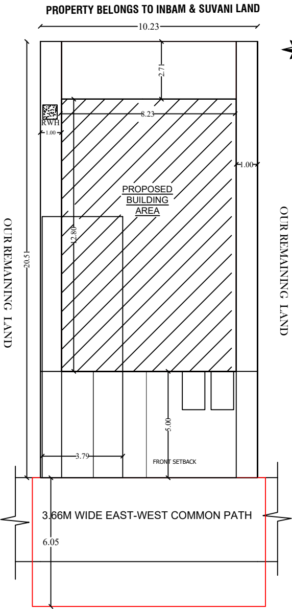
SITE PLAN
