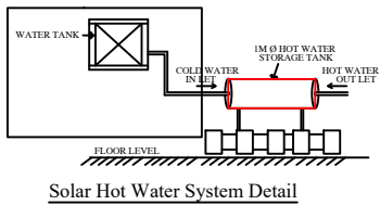
Solar Hot Water System Detail
