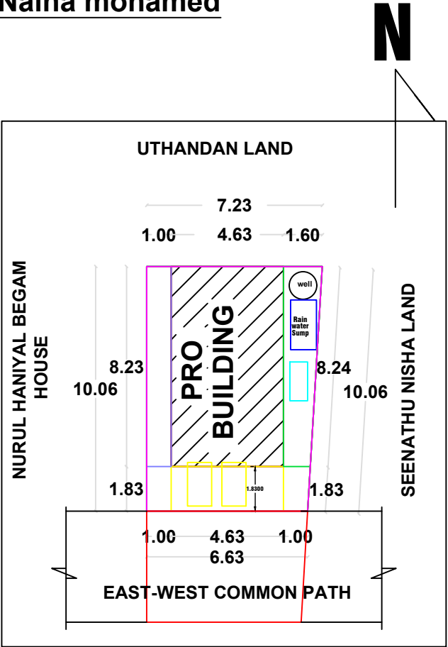
SITE PLAN & KEY PLAN (1:100)
