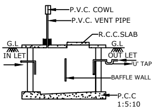
SEC. OF SEPTIC TANK
