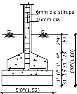
COLUMN FOUNDATION DETAIL
