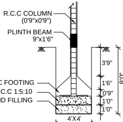
FOUNDATION DETAILS (SCALE 1" = 4'0")
