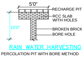
RAIN WATER HARVESTING PERCOLATION PIT WITH BORE METHOD
