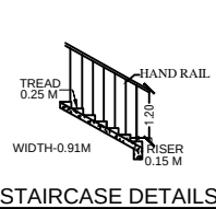
STAIRCASE DETAILS
