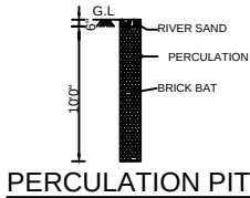
PERCULATION PIT
