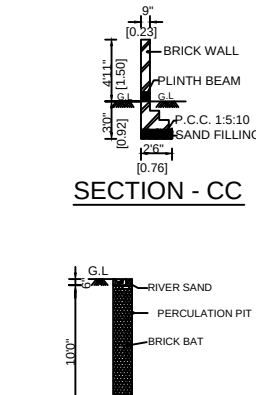
PERCOLATION PIT
