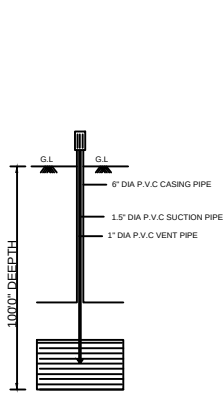
BORE WELL
