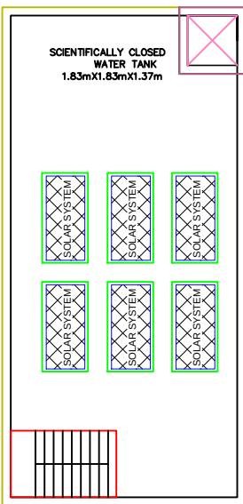
TERRACE PLAN
