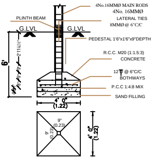
FOUNDATION DETAIL
