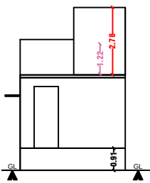
FRONT ELEVATION
