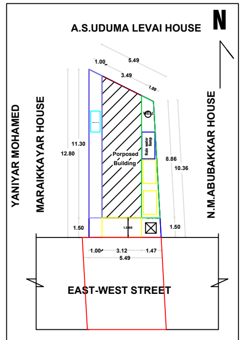
SITE PLAN CUM KEYPLAN
