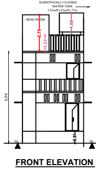
FRONT ELEVATION
