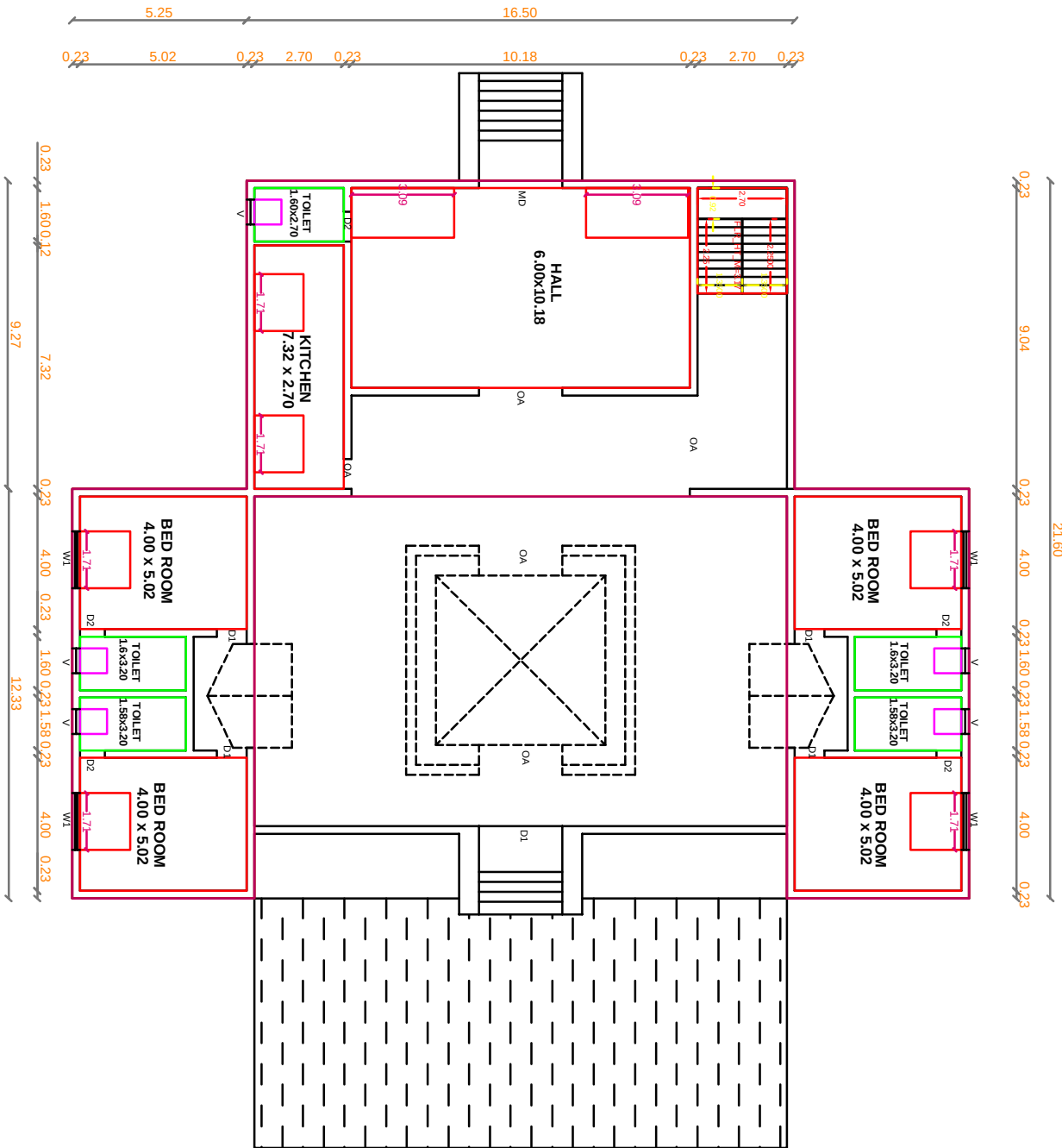
GROUND FLOOR PLAN PROPOSED
