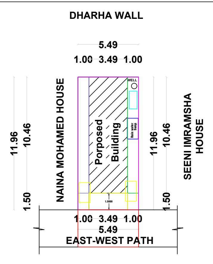
SITE PLAN CUM KEYPLAN
