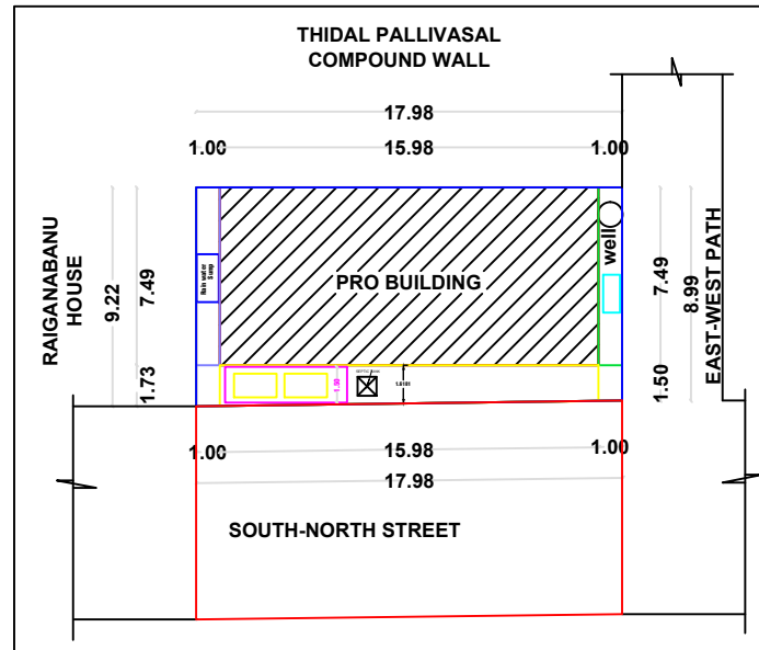
SITE PLAN & KEY PLAN
