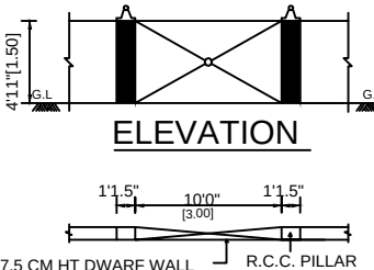
COMPOUND WALL PLAN
