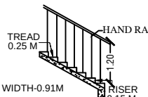
STAIRCASE DETAIL
