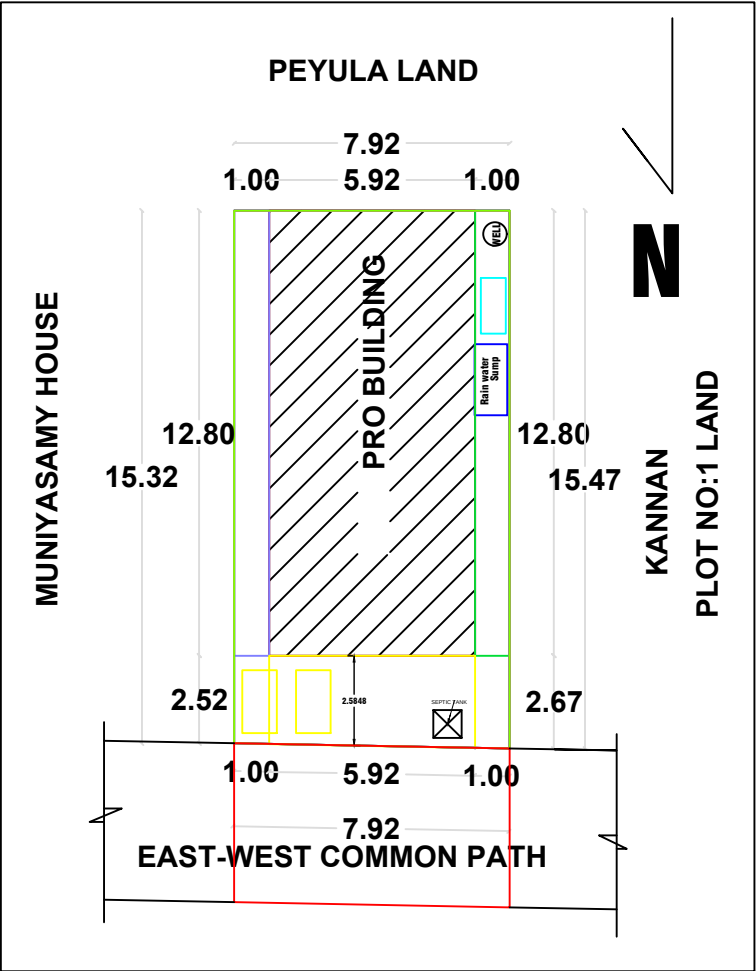
SITE PLAN & KEY PLAN
