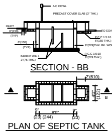
PLAN OF SEPTIC TANK
