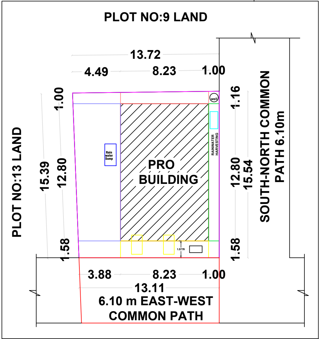
SITE PLAN & KEY PLAN (1:100)
