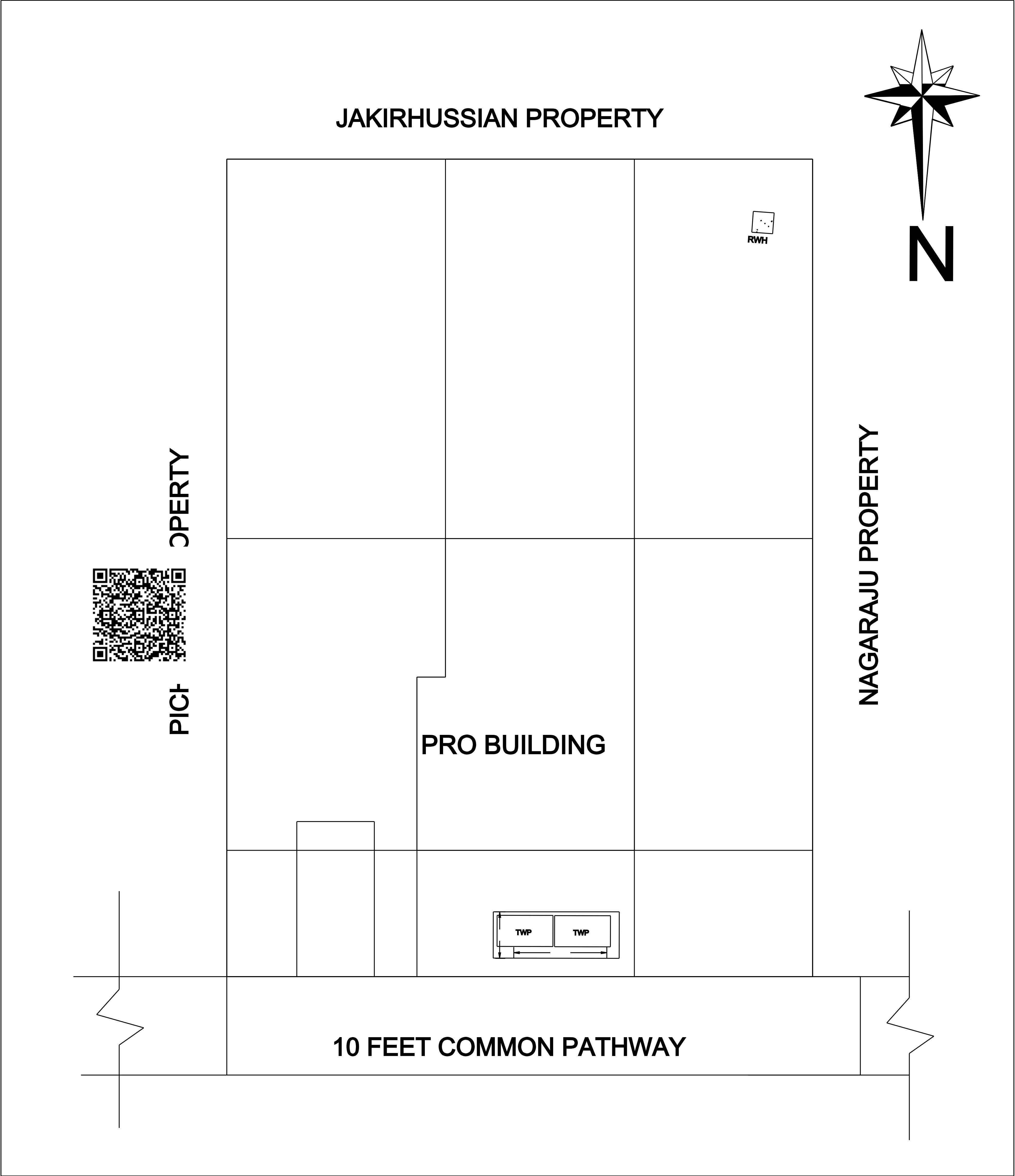
SITE PLAN
