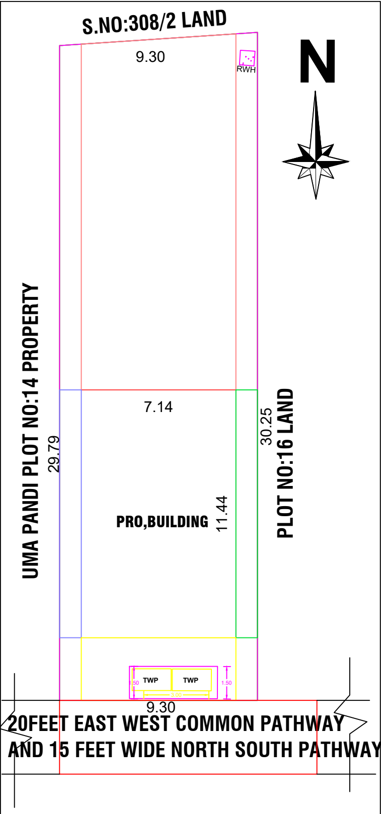
SITE PLAN
