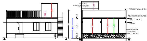
FRONT ELEVATION
