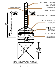
FOUNDATION DETAIL
