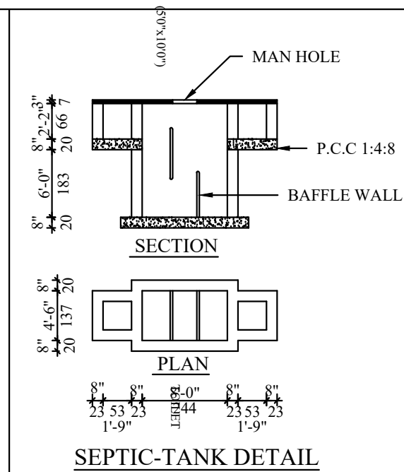
SEPTIC-TANK DETAIL
