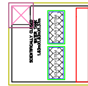
TERRACE FLOOR PLAN
