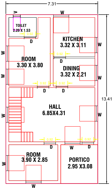
PRO., GROUND FLOOR PLAN
