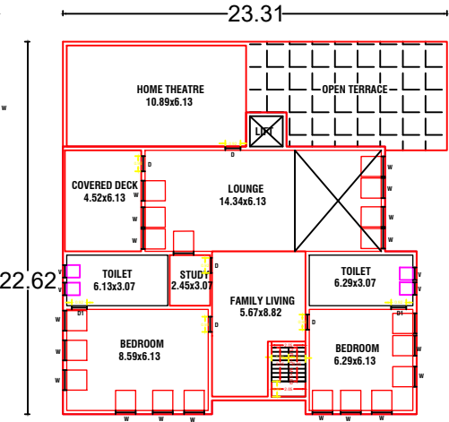
PRO., FIRST FLOOR PLAN
