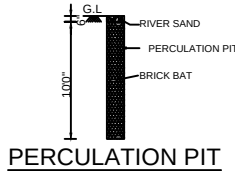
PERCOLATION PIT
