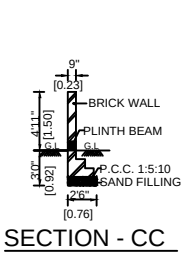
SECTION - CC
