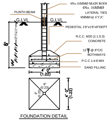
FOUNDATION DETAIL
