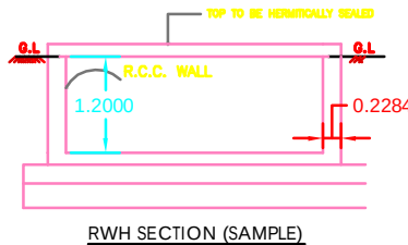
RWL_CAPACITY_L=2000LTRS
