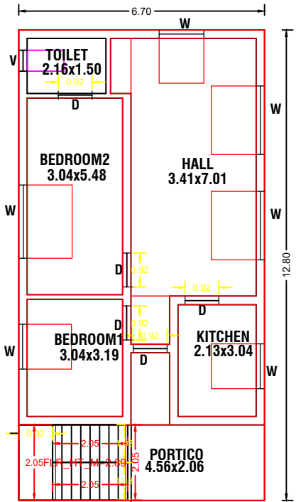
PRO., GROUND FLOOR PLAN
