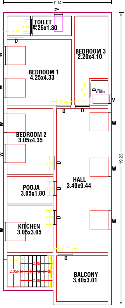
PRO., FIRST FLOOR PLAN
