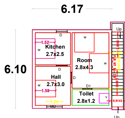
GROUND FLOOR PLAN TERRACE FLOOR PLAN
