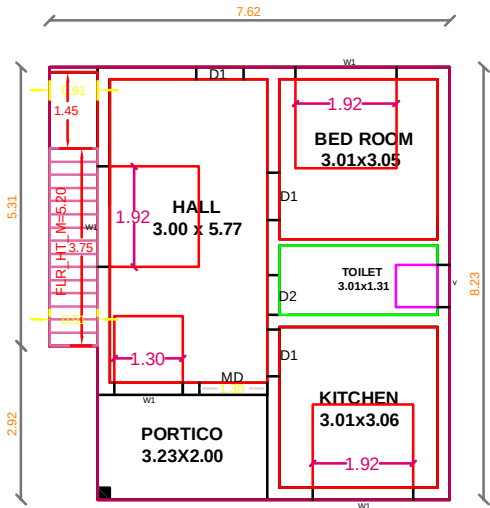
GROUND FLOOR PLAN PROPOSED
