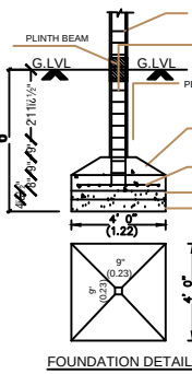
FOUNDATION DETAIL
