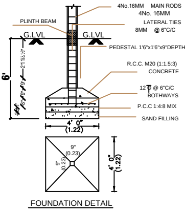
FOUNDATION DETAIL
