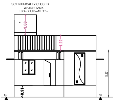
FRONT ELEVATION
