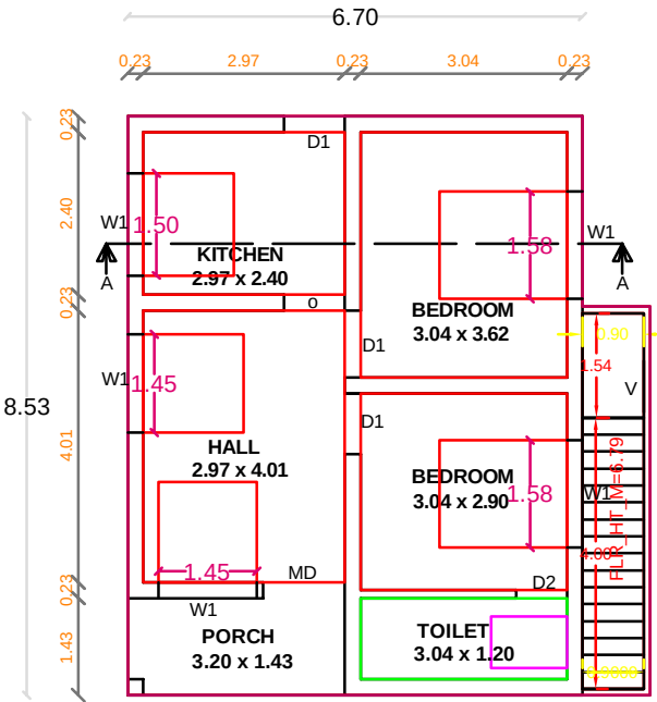
GROUND FLOOR PLAN PROPOSED
