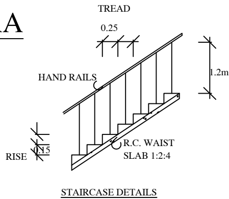
STAIRCASE DETAILS
