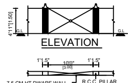
COMPOUND WALL PLAN
