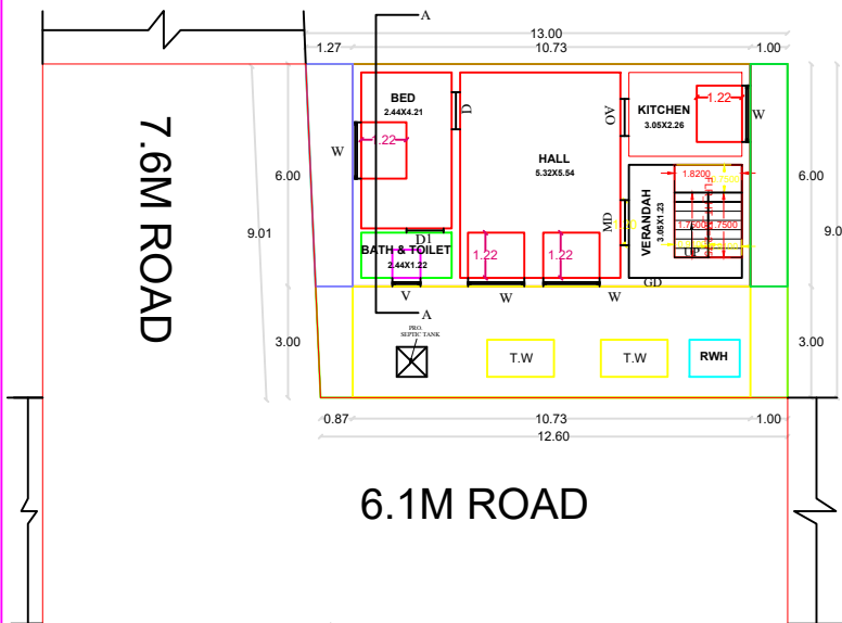
SITE PLAN CUM GROUND FLOOR PLAN
