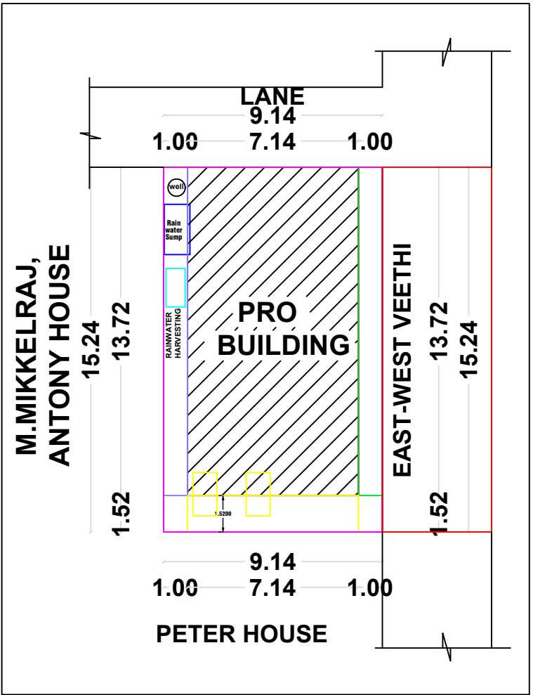
SITE PLAN & KEY PLAN (1:100)
