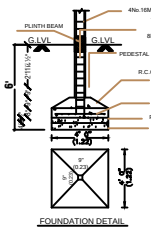
FOUNDATION DETAIL
