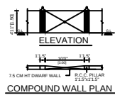
COMPOUND WALL PLAN
