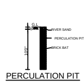
PERCOLATION PIT
