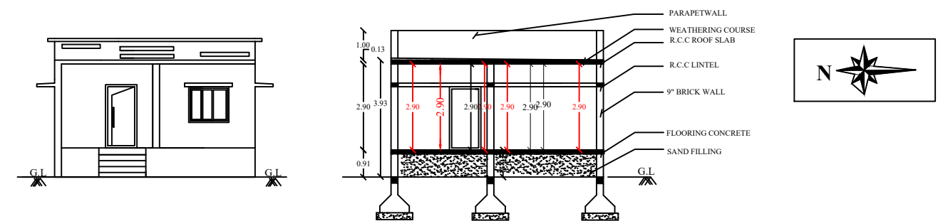
FRONT ELEVATION SECTION ON - "A-A"
