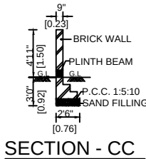
SECTION - CC
