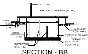
SECTION - BB PLAN OF SEPTIC TANK
