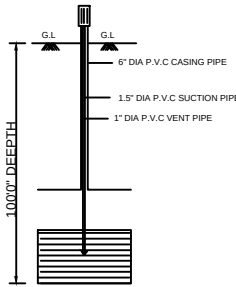
BORE WELL
