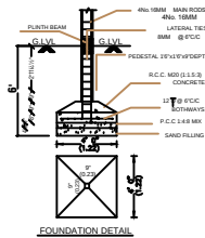
FOUNDATION DETAIL
