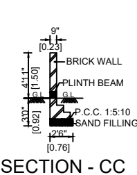
SECTION - CC
