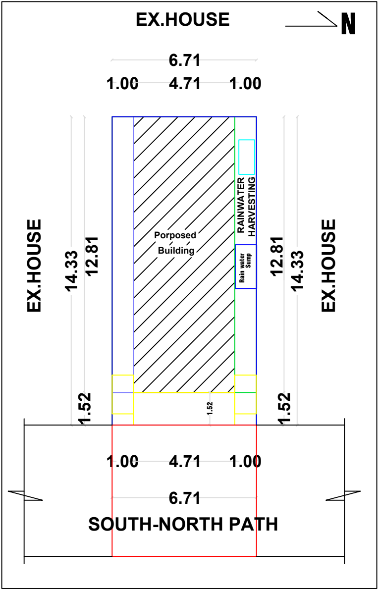
SITE PLAN CUM KEYPLAN
