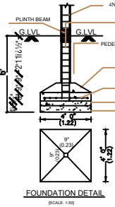
FOUNDATION DETAIL
