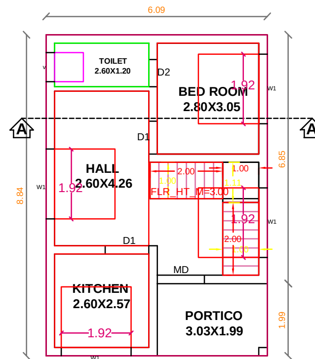
GROUND FLOOR PLAN PROPOSED
