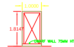
WIKET GATE ELEVATION
