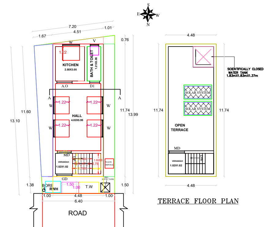
SITE PLAN CUM GROUND FLOOR PLAN
