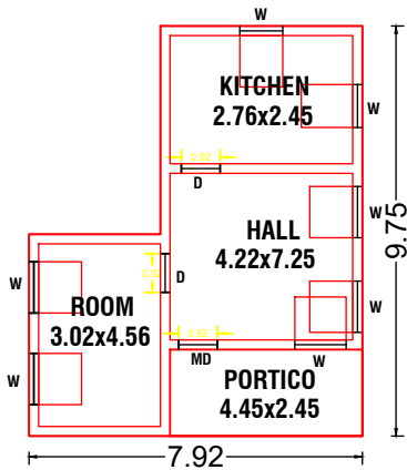
PRO., GROUND FLOOR PLAN
