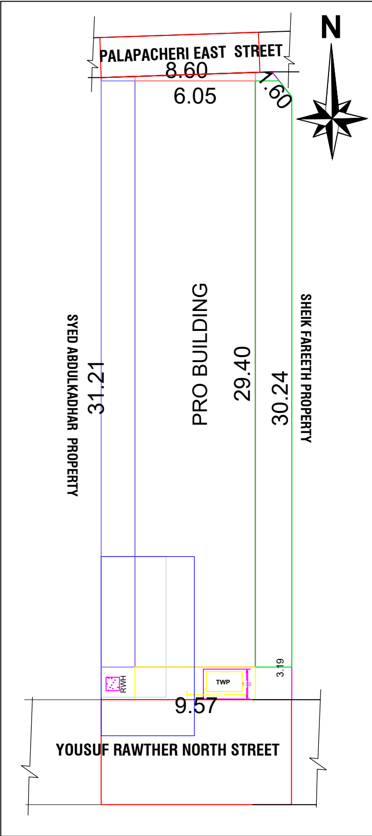
SITE PLAN
